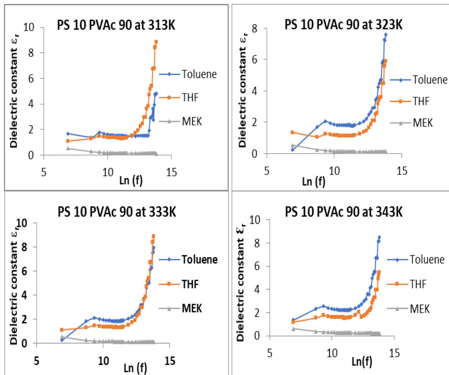
Fig. 2 (b): Variation between frequency and dielectric constant for blends in different solvent at constant temperatures.
