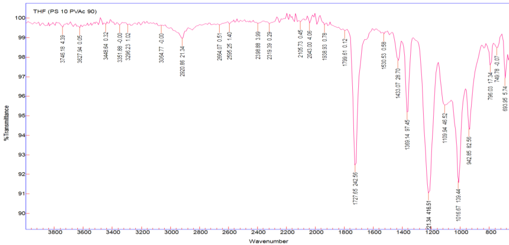
Fig.1 (b): FTIR PS (10) +PVAc (90) (THF)
