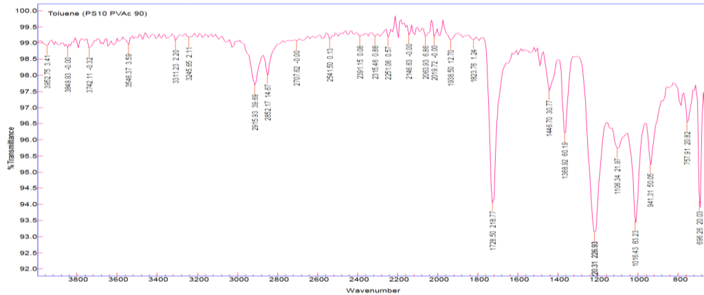
Fig.1 (c): FTIR PS (10) +PVAc (90) (Toluene)
