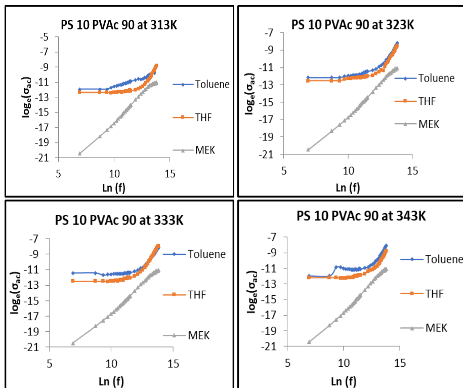
Fig. 2 (a): Variation between frequency and a.c. conductivity for blend in different solvent at constant temperatures.
